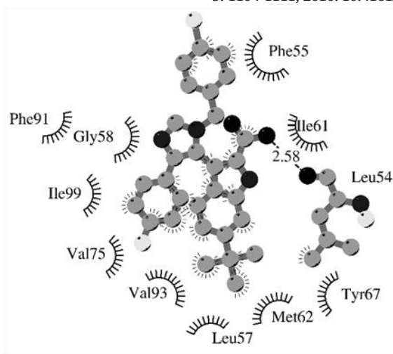
Figure Intermolecular interactions between compound A and human MDM2 protein. The hydrophobic forces are shown as arches and the hydrogen bonds as a line
