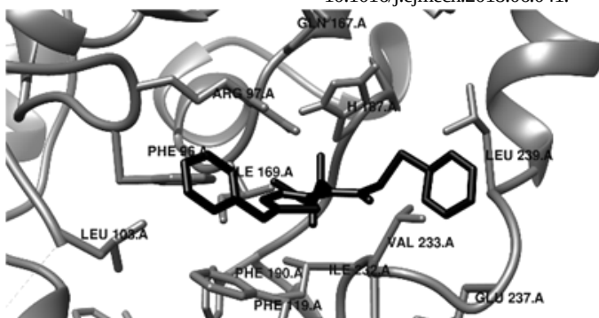
Figure 1. The binding mode of the most potent compound
