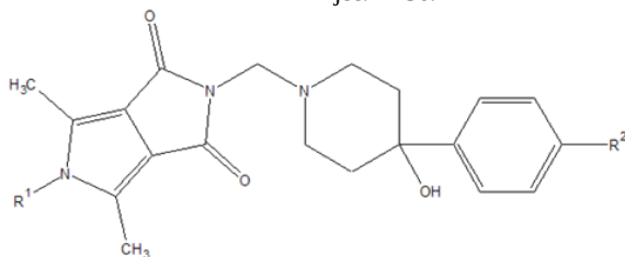
Figure 1. General formula of obtained compounds
