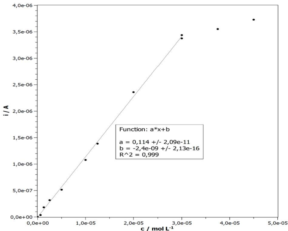
Figure 1 Calibration curve
