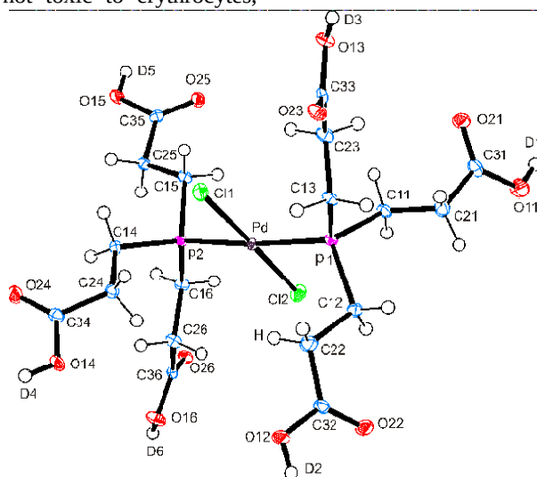
Fig. 1. Molecular structure of palladium(II) complex with tris(2-carboxyethyl)phosphine – PdTCEP [1]
