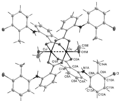
Figure. Crystal structure of [\text{Cu}_2(\text{C}_{56}\text{H}_{44}\text{Cl}_4\text{N}_4\text{O}_8)(\text{CH}_3\text{OH})_2]
