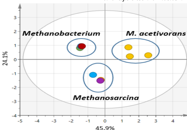
Fig. 1. PCA score plot of methanogenic archaea
